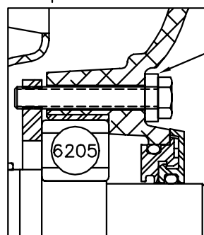
PULLEY END DETAIL
