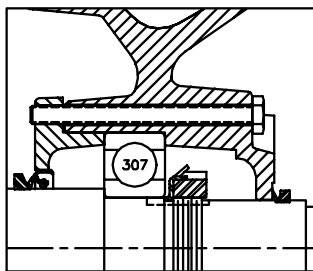
PULLEY DETAIL
