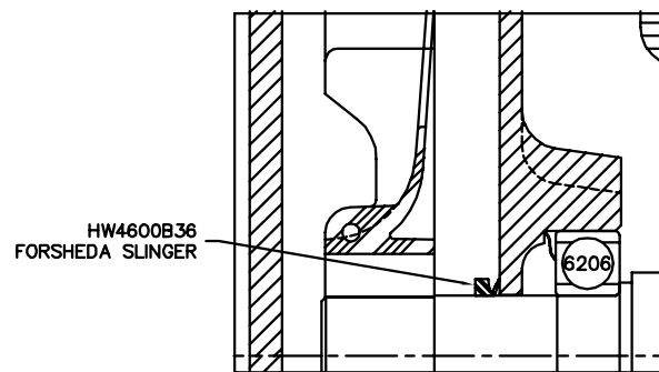
FRONT END DETAIL
