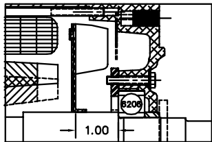
PULLEY END DETAIL
