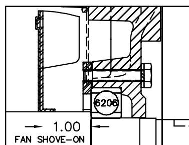
PULLEY END DETAIL
