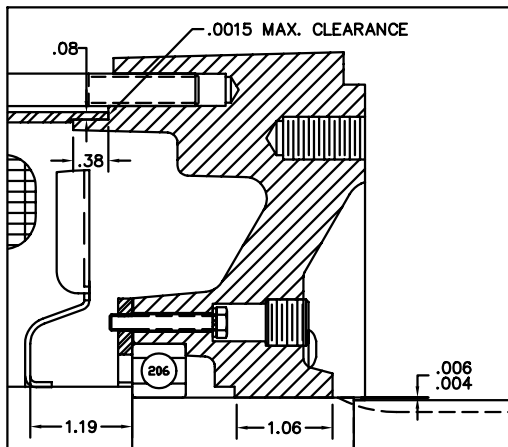
PULLEY END DETAIL
