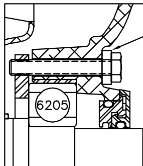
PULLEY END DETAIL
