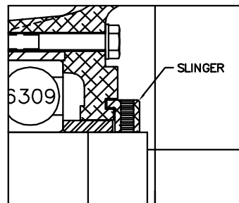
PULLEY END DETAIL
