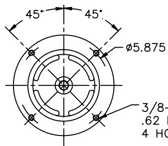
FRONT FACE DETAIL (COVER REMOVED)
