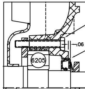
PULLEY END DETAIL
