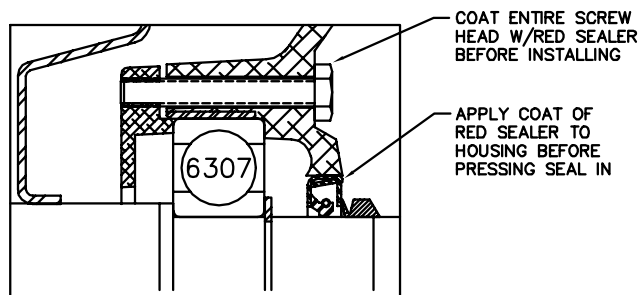
PULLEY END DETAIL
