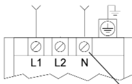
208/240 Vac SINGLE PHASE INPUT (WHERE APPLICABLE)
